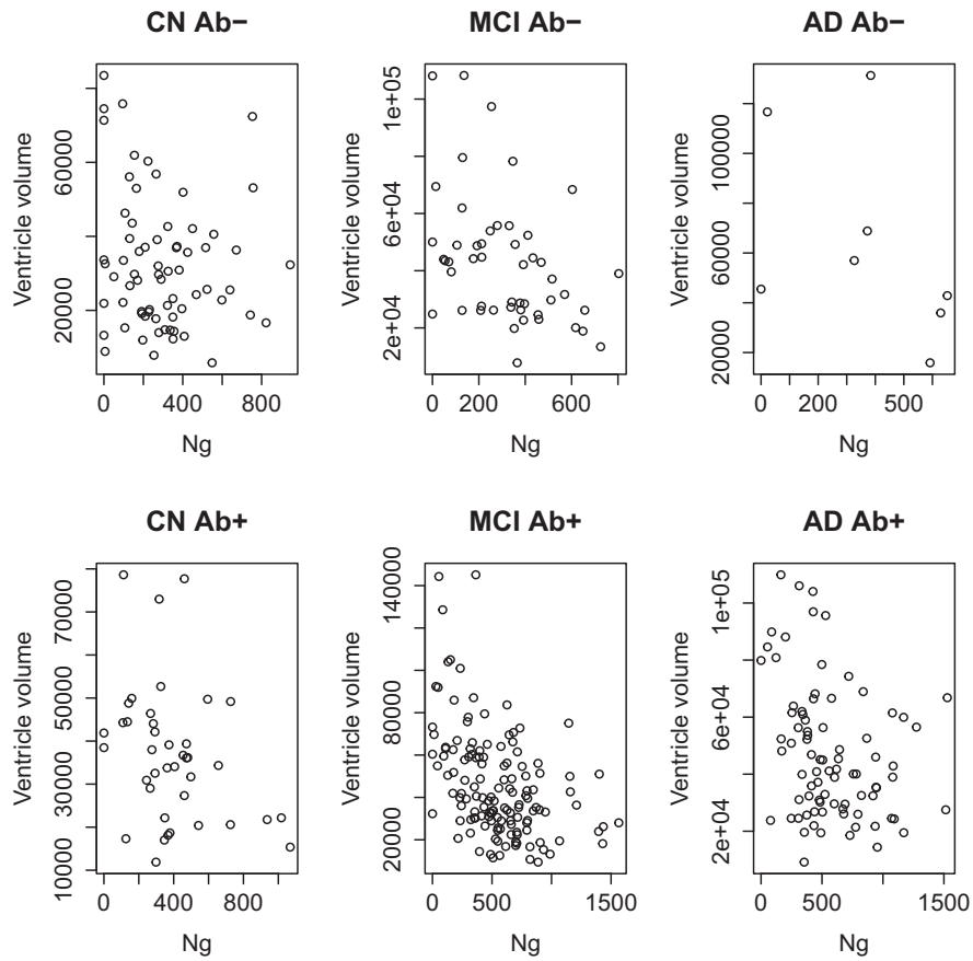
Figure EV2. CSF Ng and ventricular volume. Scatter plots showing CSF Ng (ng/l) and ventricular volumes (ml) in different diagnostic group, separately for Aβ-negative (upper row) and Aβ-positive subjects (lower row). The plots illustrate the general observation that very high CSF Ng levels are often seen in subjects with relatively small ventricles, independent of diagnostic group and Aβ status.
