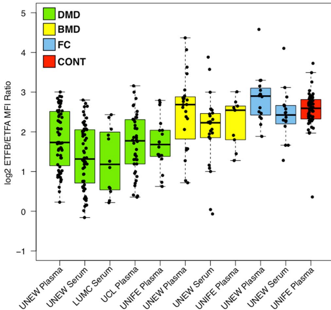
Supplementary Figure S6. Varying ETFB/ETFA ratios in plasma/serum of NMD patients and control groups. Boxplots represent the ETFB/ETFA signal ratio in plasma/serum of NMD patients and control groups, where green, yellow, blue and red boxes represent DMDs, BMDs, female carriers and controls, respectively. For each sample group, the box-and-whisker plot represents signal ratio within lower and upper quantile (box), the median (horizontal line within box), percentiles of 5% and 95% (whiskers) and outliers (dots).
